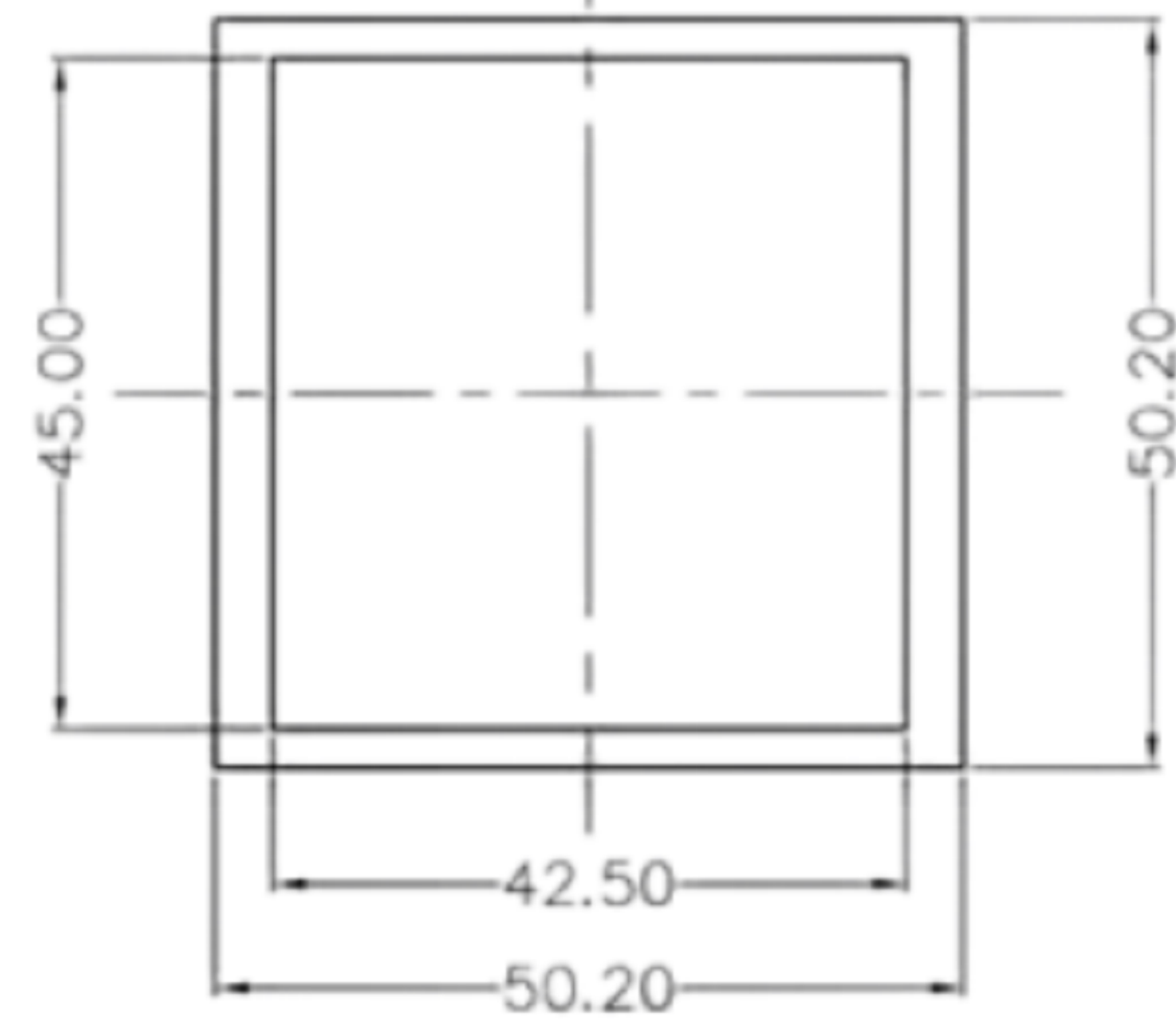
PANEL CUT-OUT
